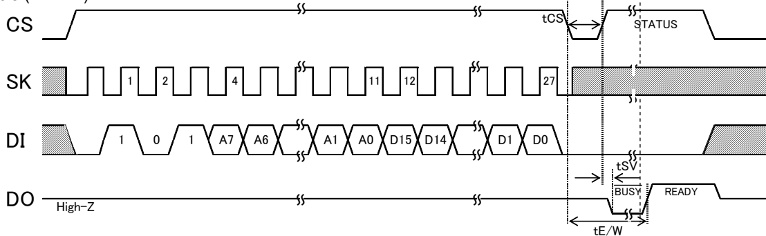
Fig.26 Write cycle
