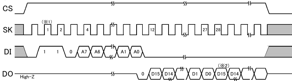
Fig.25 Read cycle
